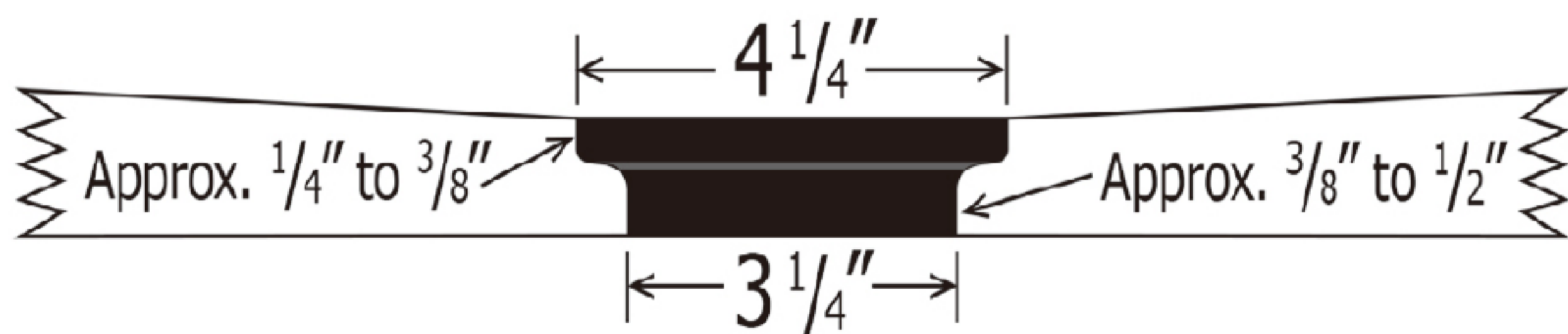
Drain Detail:
